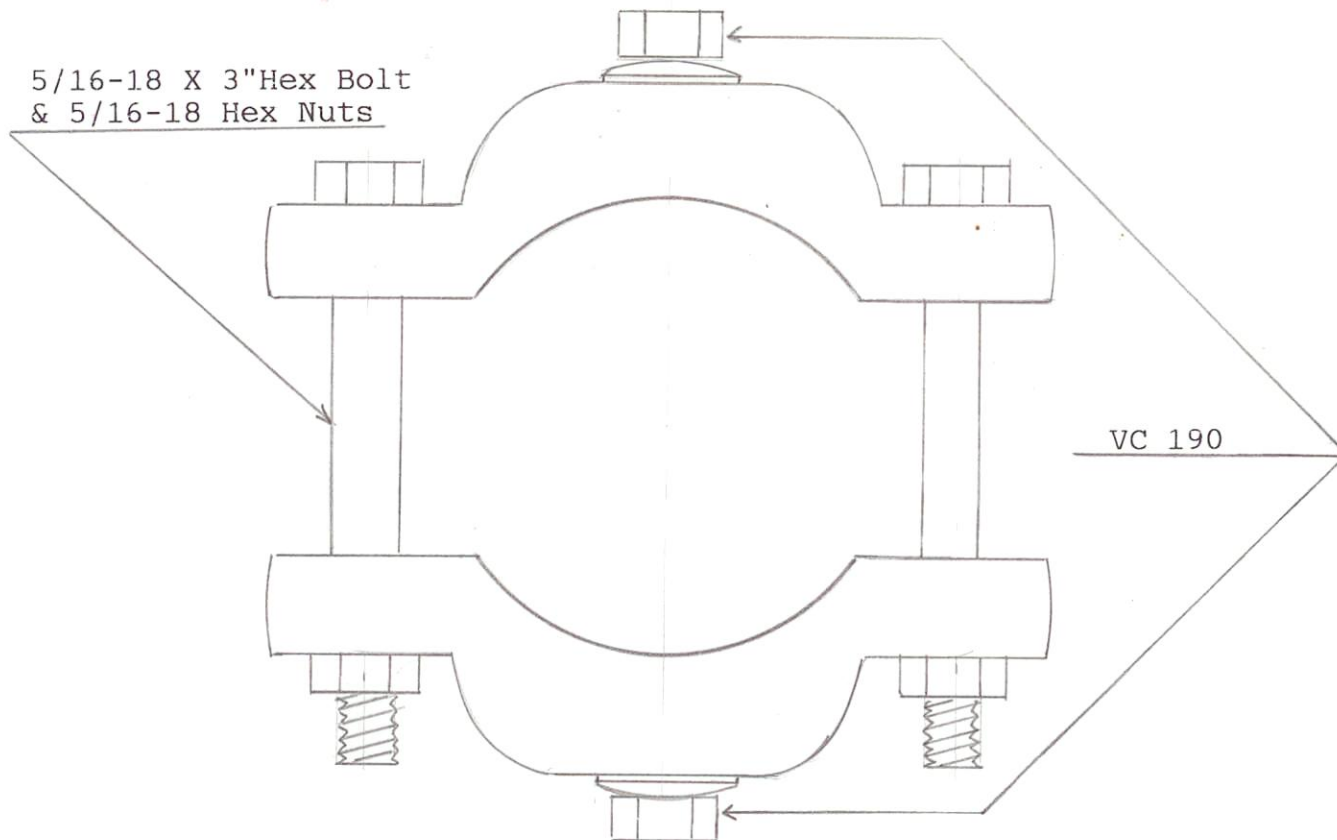
STANDARD VCS 212-2 ASSEMBLY (DOUBLE SADDLE OPTION)
